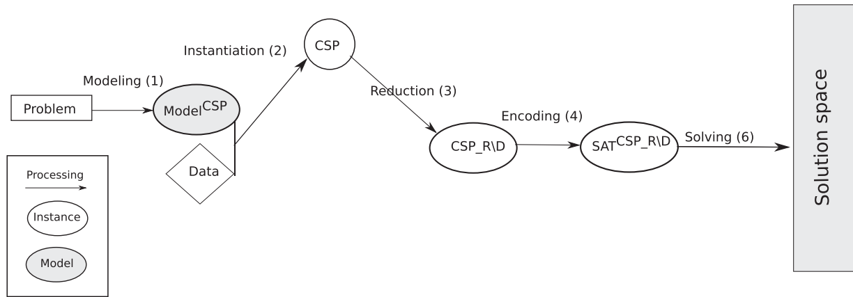
Fig. 3. Best solving chain.
