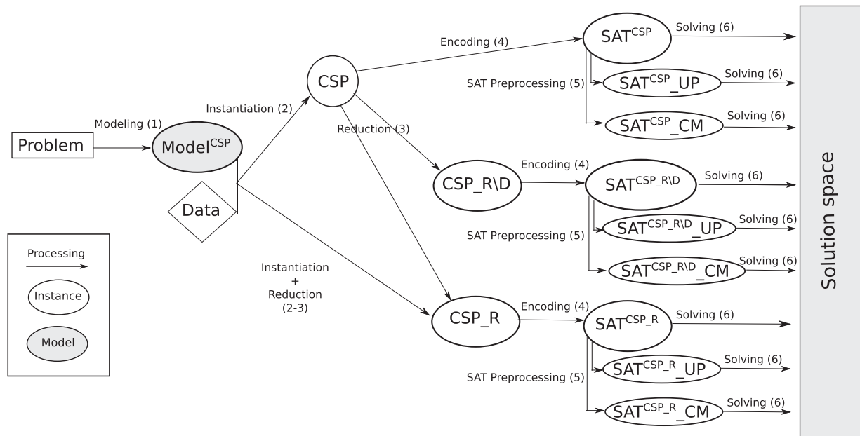
Fig. 1. Models, instances, and their processing.
