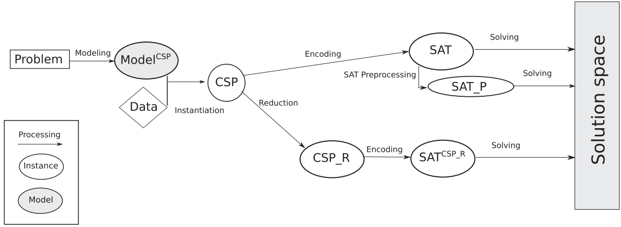
Fig. 2. Models, instances, and processing presented in Lardeux et al. (2015).
