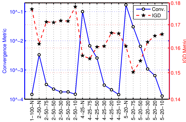
Fig. 4. Average performance of PGA for the 5-objectives DTLZ1 problem. The solid blue line with circle marks corresponds to results for the convergence metric, while the dotted red line with star marks refers to IGD.
