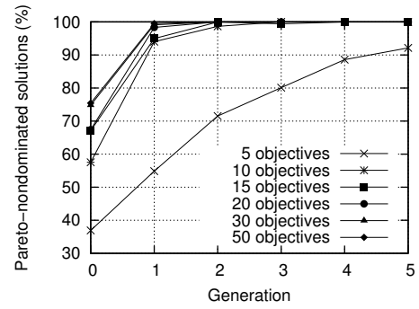
Fig. 1. Proportion of Pareto-nondominated solutions.
